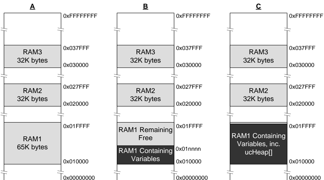
Figure 8 Memory Map
