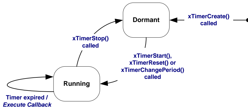
Figure 39 Auto-reload software timer states and transitions
