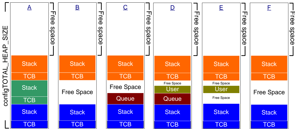
Figure 7. RAM being allocated and freed from the heap_4 array
