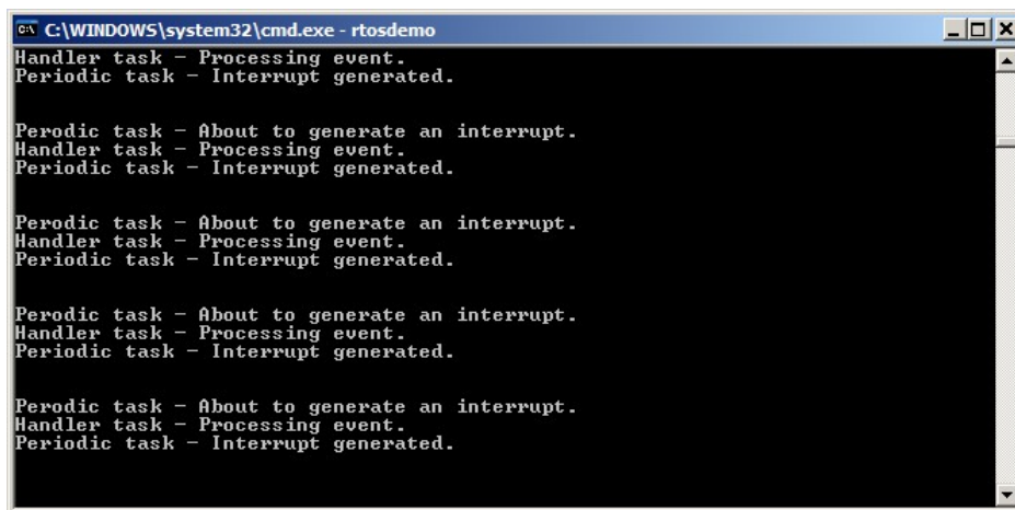
Figure 78. The output produced when Example 16 is executed
